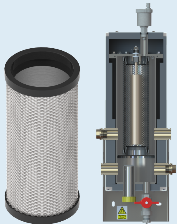
Cross-section showing upper chamber with magnets, before descending into the actual particle filter and anode chamber.
